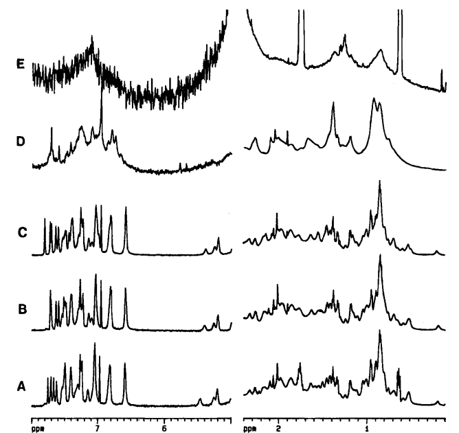
FIGURE 7: Comparison of 1D ^1H NMR spectra between p16/Δ1-8 WT and mutants, in D_2O at 600 MHz: (A) WT; (B) D84N; (C) D84H; (D) P114L; (E) G101W. Increased vertical scale (10–12 times) was used for the spectra of the aromatic region (left) compared to those of the aliphatic region (right). The sharp resonance at 0.64 ppm in A is arising from an impurity in the chemical shift standard DSS. The intense lines at 0.60 and 0.72 ppm in E are originated from the excess buffers.
