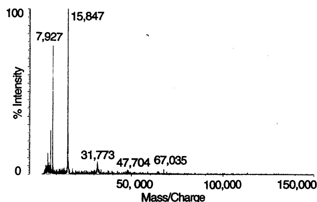
FIGURE 1: MALDI-TOF mass spectrum of p16/ \Delta 1-8. The sample contained 10 \mu M p16/ \Delta 1-8 in 0.2 mM HEPES (pH 7.0) and 50 \mu M DTT.
