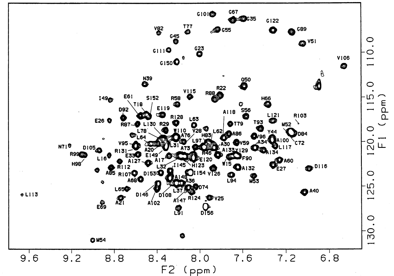
FIGURE 5: ^{15}\text{N} – ^1\text{H} HSQC spectrum of p16/ \Delta 1–8 at 600 MHz. The assignments are labeled by the one-letter code of amino acids accompanied by a sequence number.
