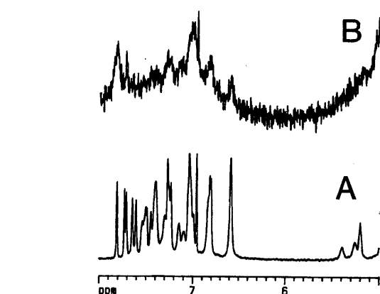
FIGURE 10: Illustration of the tendency toward aggregation of D84H by NMR. Freshly prepared D84H sample was used for the spectrum A; spectrum B was obtained after incubating the sample at room temperature for 2 days.
