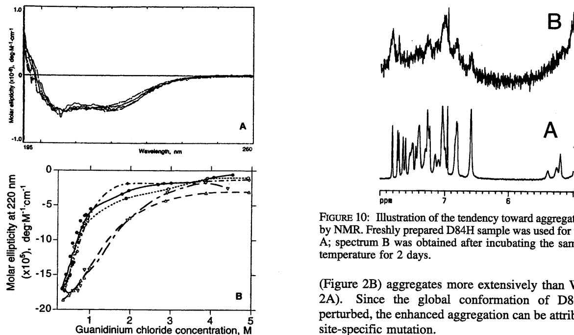
FIGURE 9: (A) Comparison of CD spectra between p16/Δ1-8 WT and mutants: (—) wild type; (---) D84N; (---) D84H; (---) P114L; (---) G101W. (B) Denaturation curves of mutants: (●) wild type; (◇) D84N; (○) D84H; (△) P114L; (▽) G101W.
